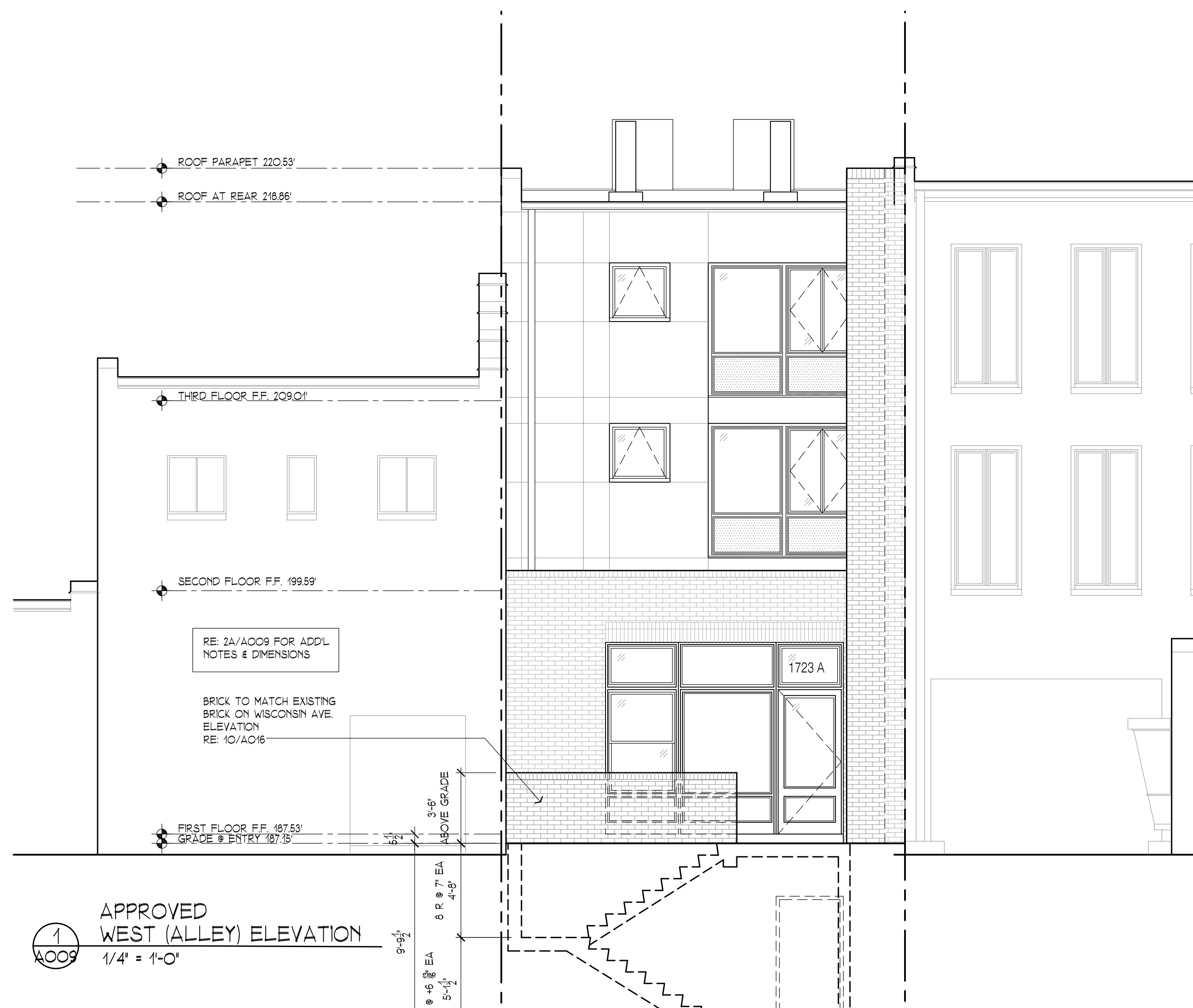
Approved Elevation
