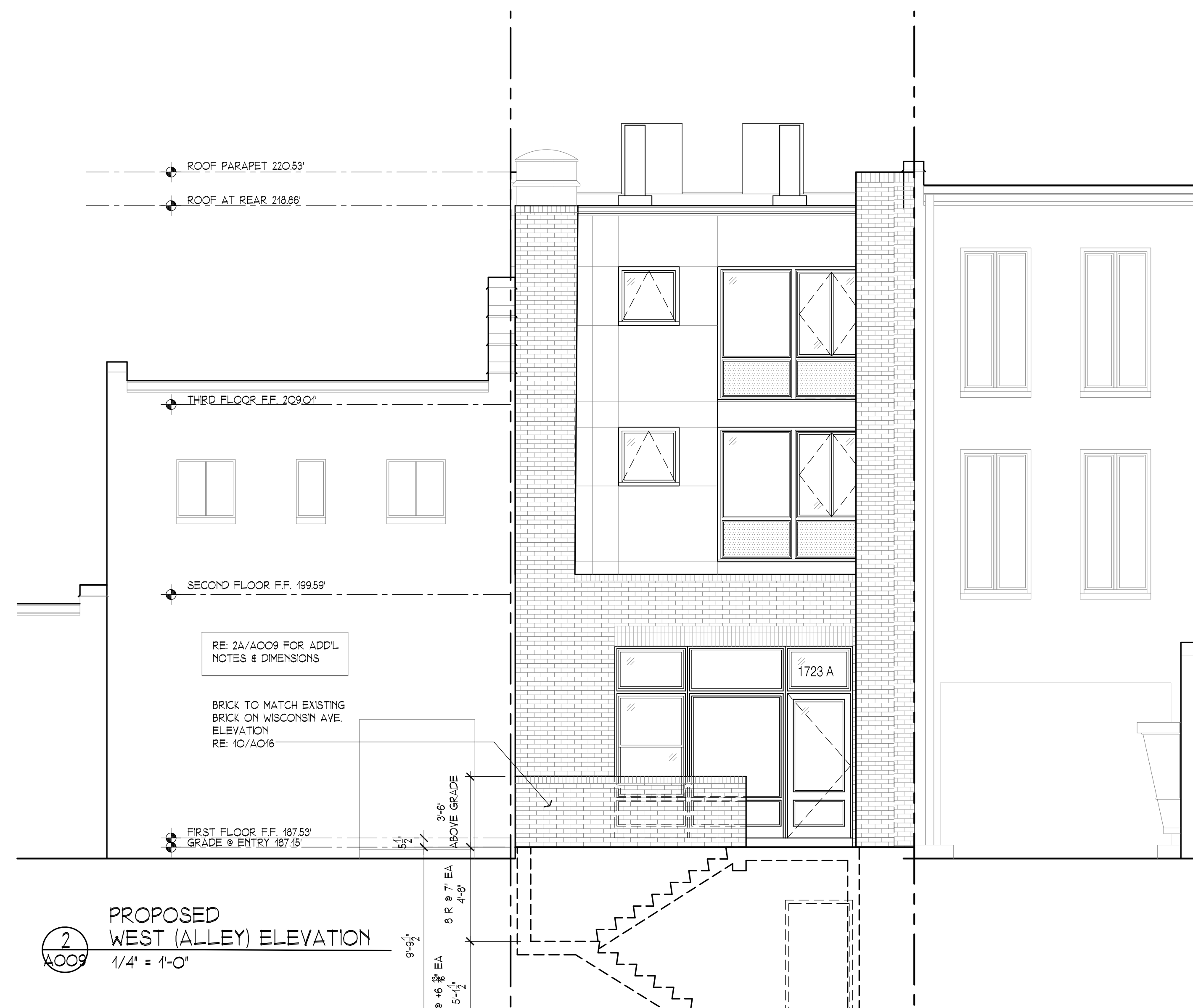
Proposed Elevation
