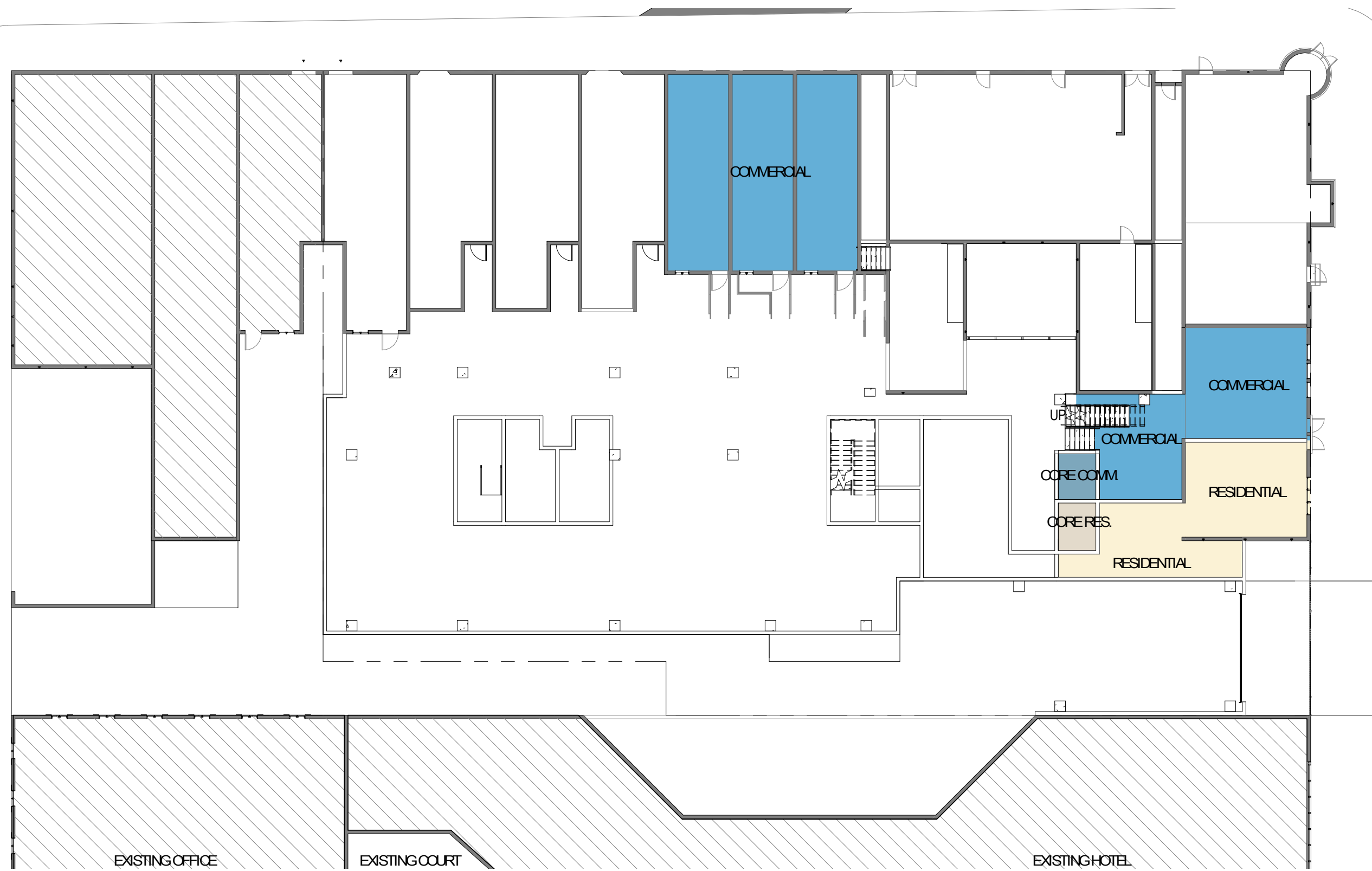
MEZZANINE LEVEL - 29TH STREET - PLAN
