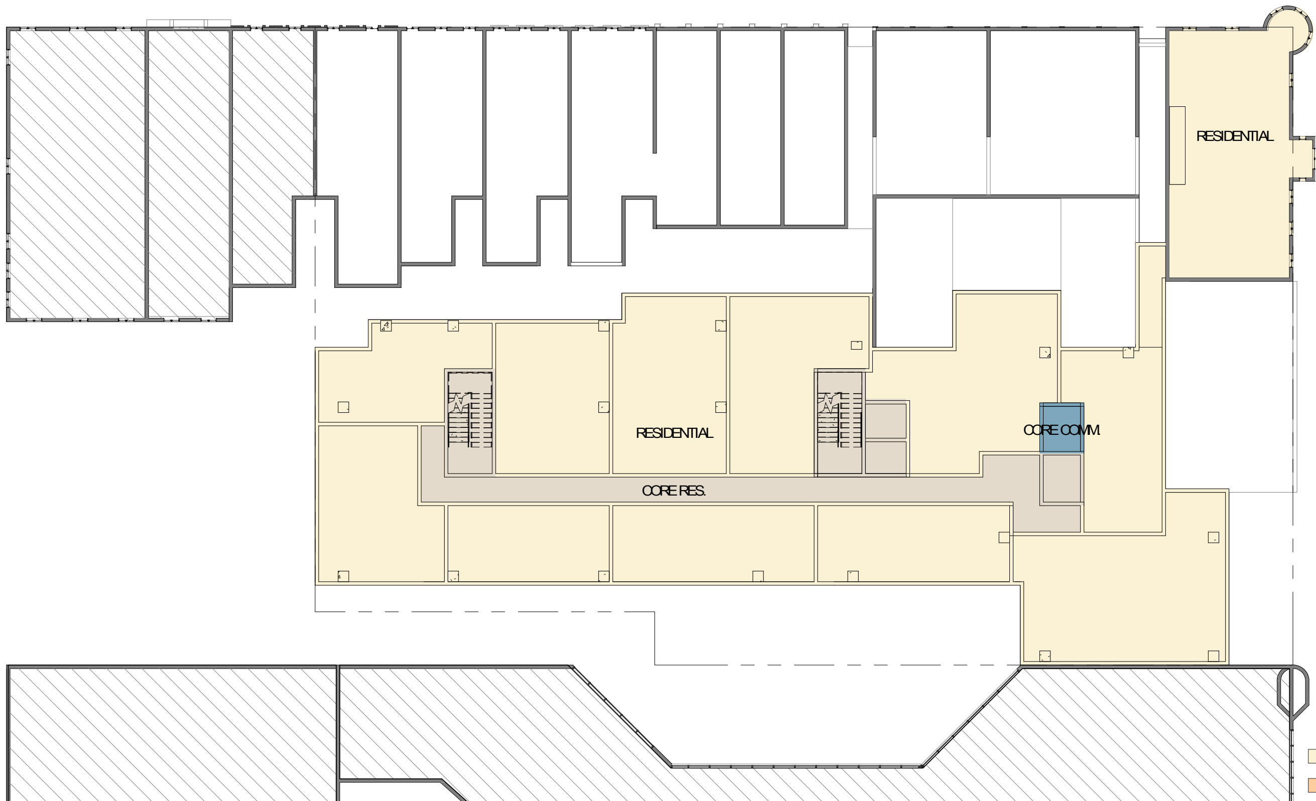
LEVEL 03 - PLAN
