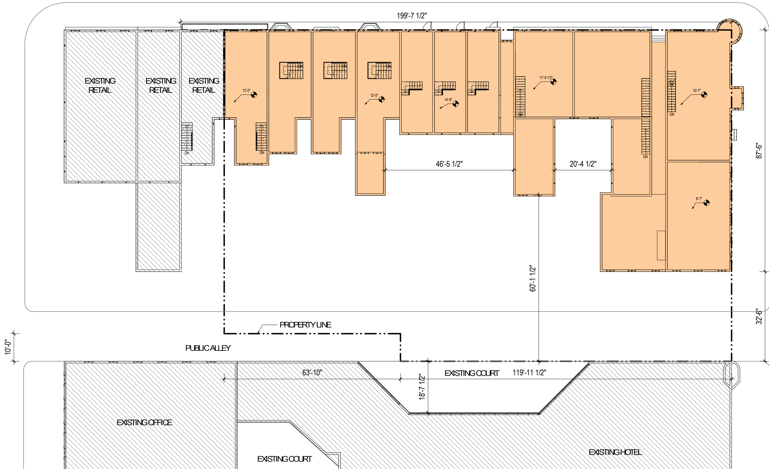
LEVEL 2 AT M ST. - EXISTING FLOOR PLAN
