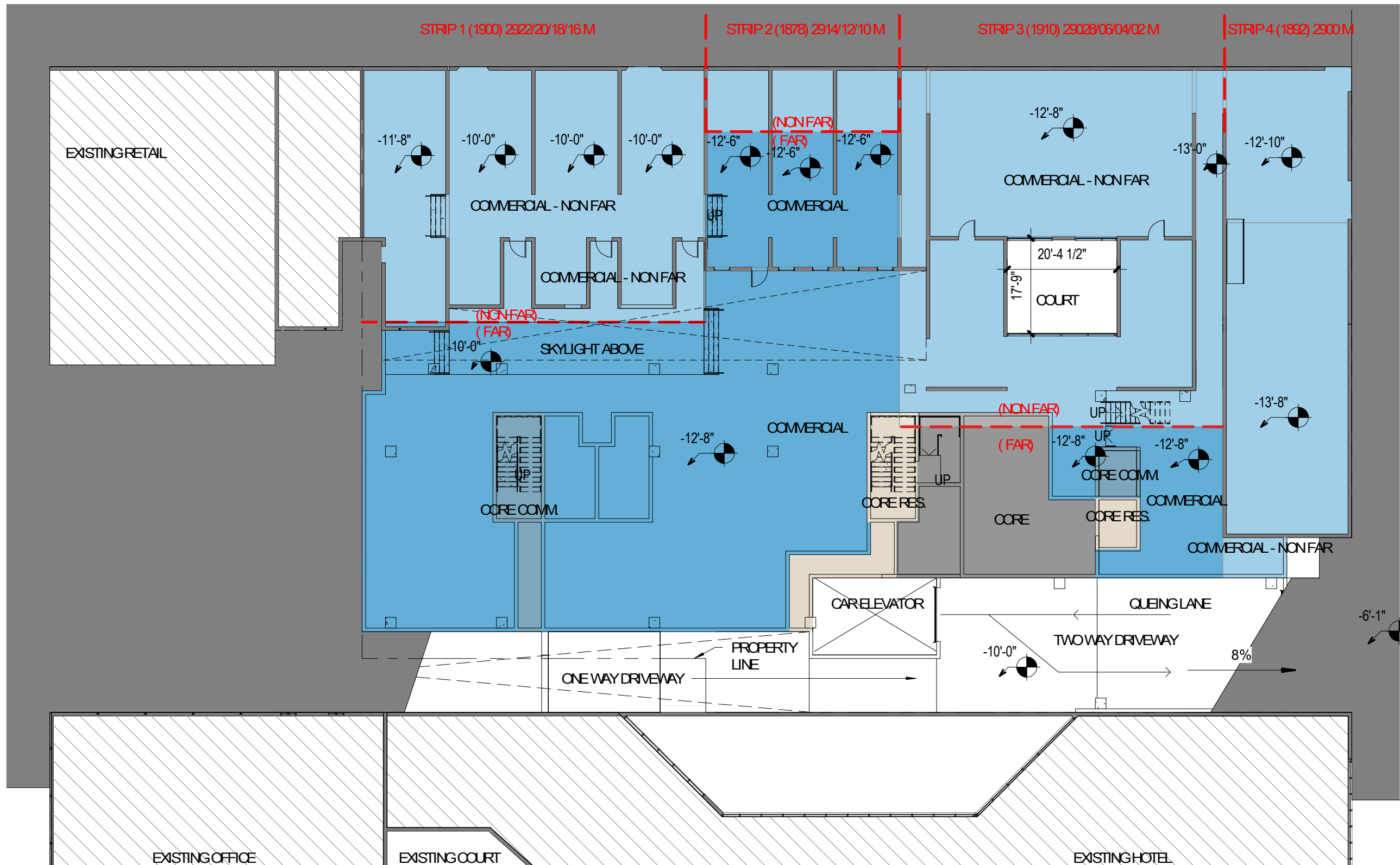
LOWER LEVEL - ALLEY - PLAN
