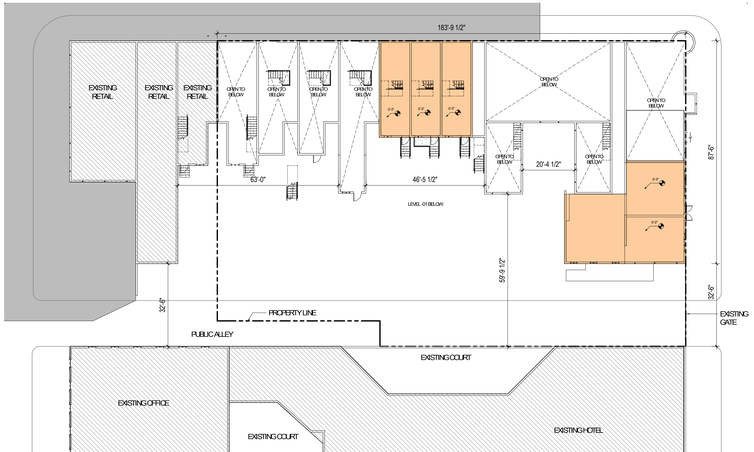
INTERMEDIATE GROUND LEVEL AT 29TH ST. - EXISTING FLOOR PLAN
