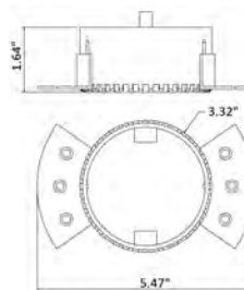
Trimless Round
