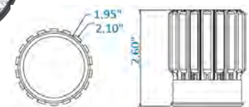
LED Engine
