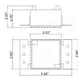
Trimless Square
