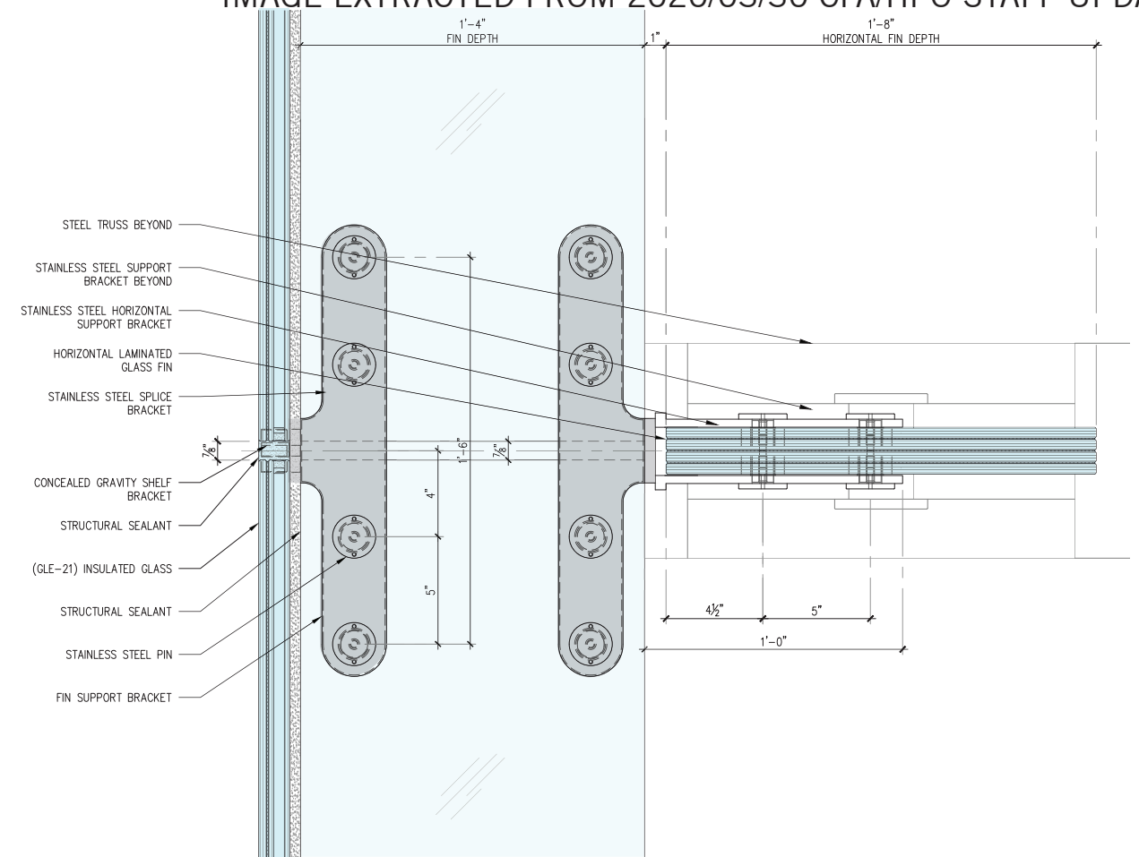
DETAIL OF GLAZING SYSTEM: VERTICAL AND HORIZONTAL FIN CONNECTION
